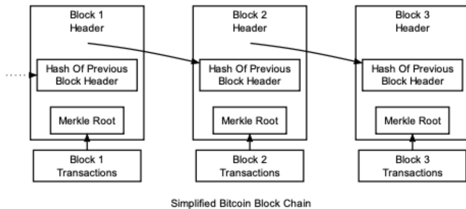
Fig.1: Simplified Bitcoin Blockchain 1
